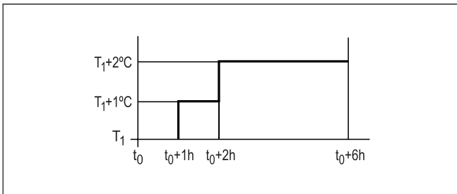
Fig. 7.19 Working method of the SLEEP function in COOL, DRY mode.
