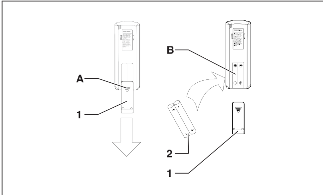
Fig. 6.1 Fitting the remote controller batteries.
