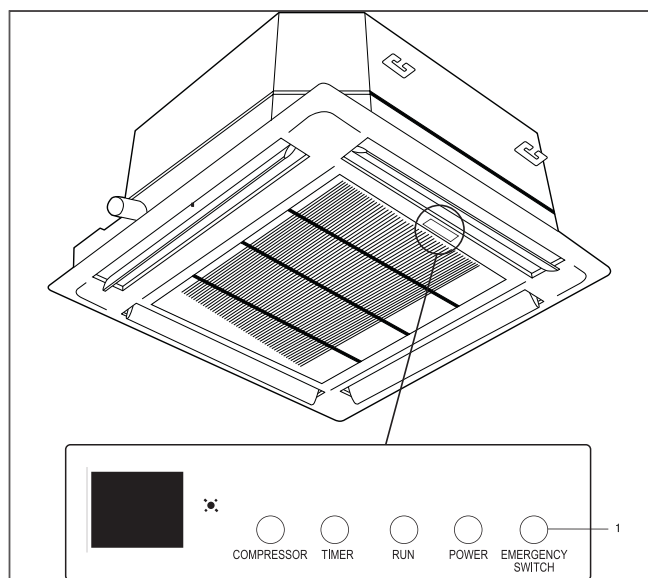
Fig. 9.1 Emergency operation/operation test switch.
