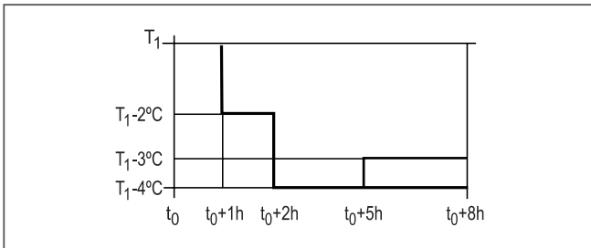
Fig. 7.20 Working method of the SLEEP function in HEAT mode.
