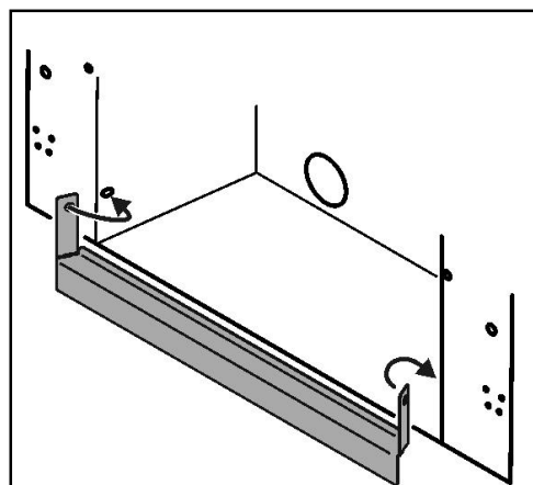
Figure 1. Baffle fitting (Shown without burner for clarity)
